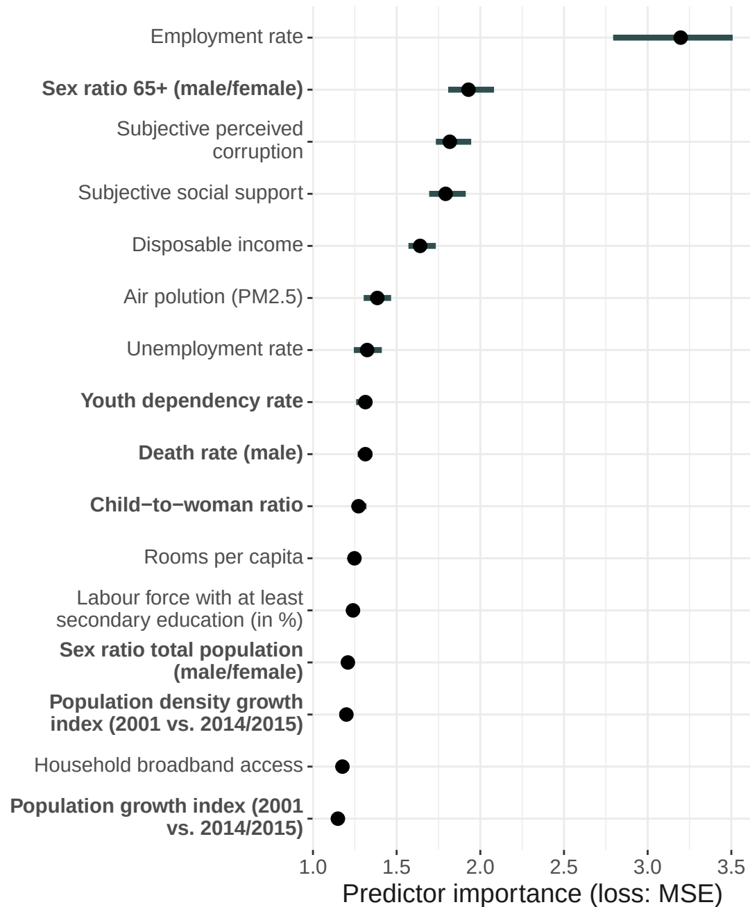
Random Forest
