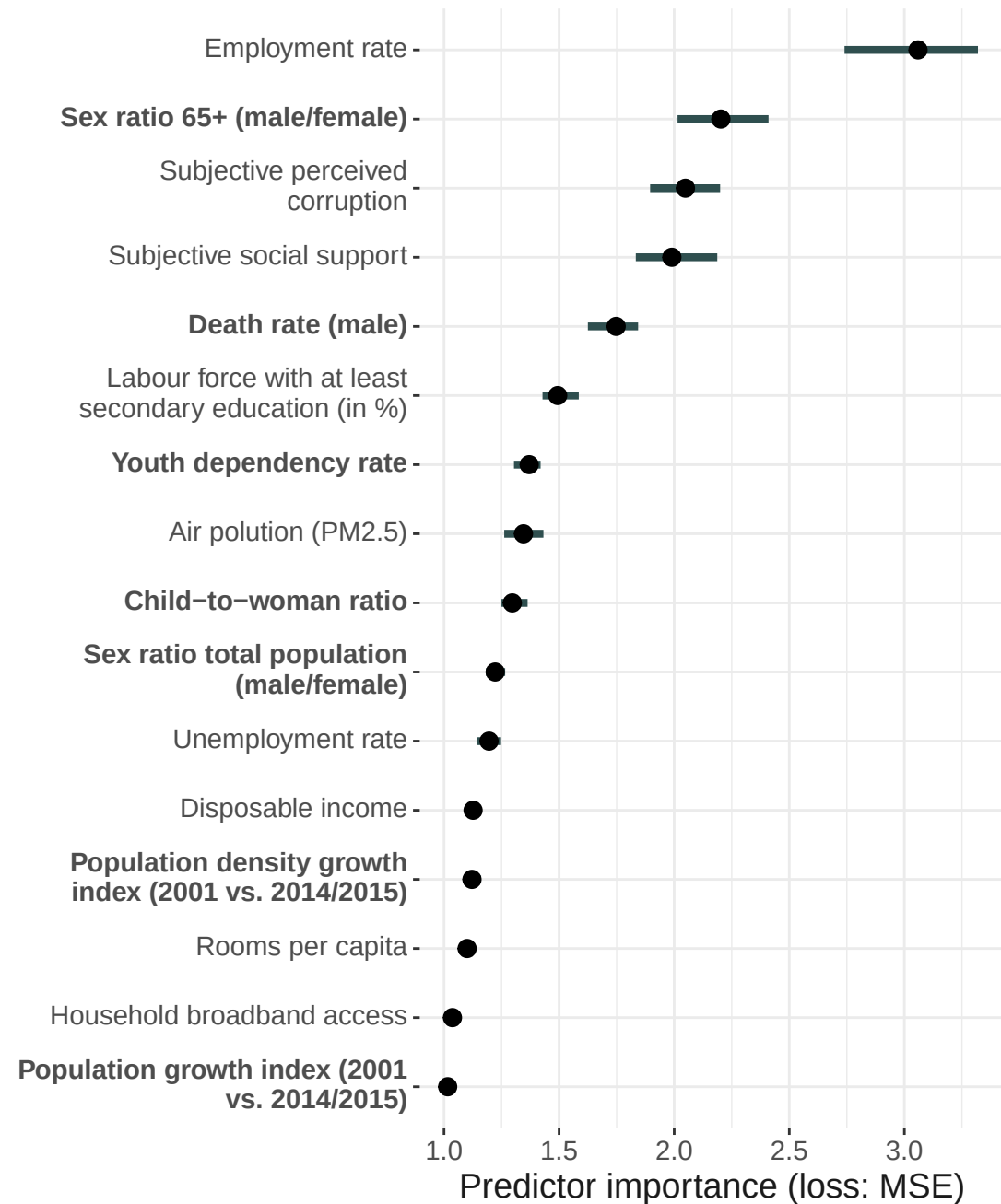
XGBoost
